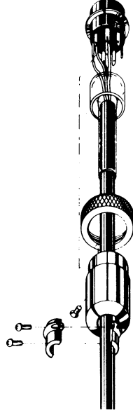
Microphone plug exploded view
